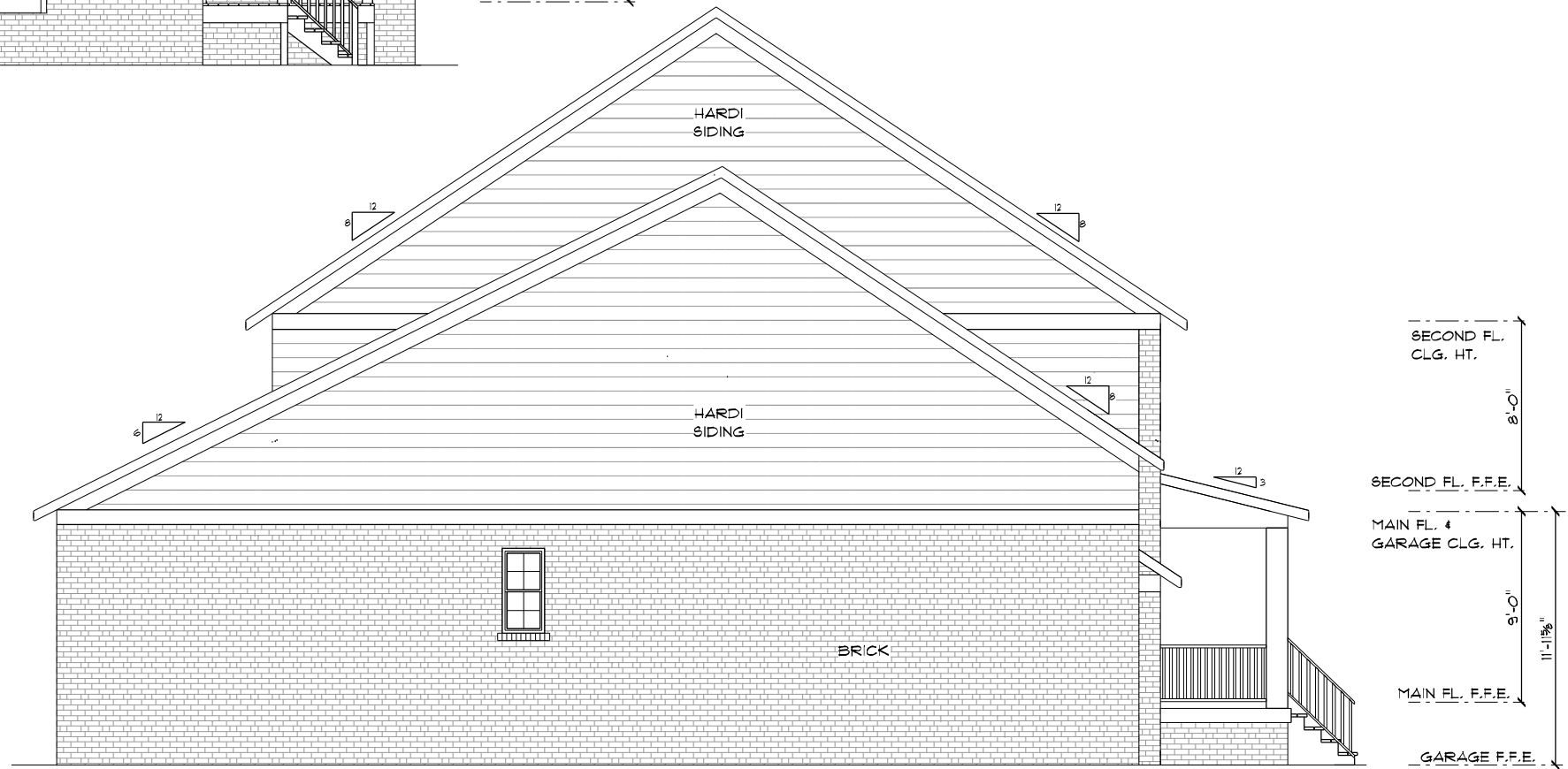
LEFT ELEVATION
